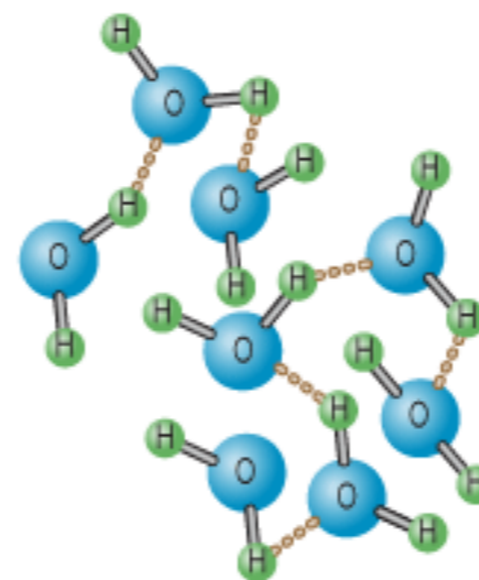
Structure of molecules in water
