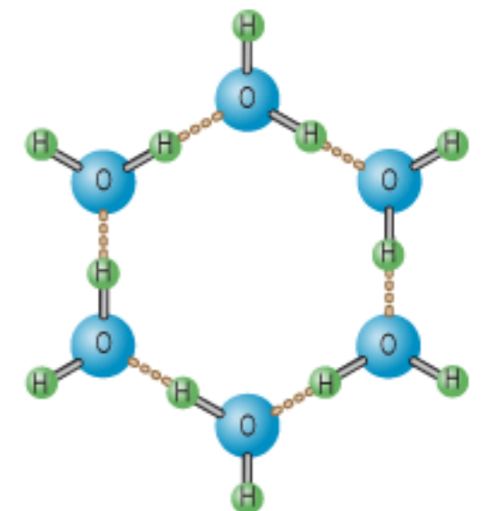
Structure of molecules in ice
